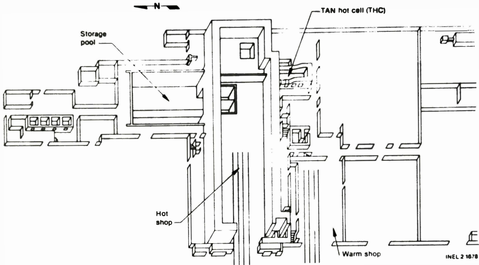
Figure 2. TAN-6U7 building showing the TAN Hot Shop, Hot Cell (THC), and storage pool.
