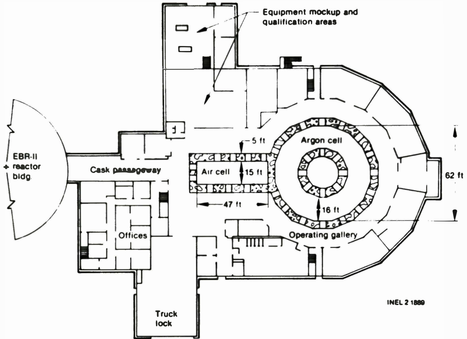
Figure 15. Plan view of HFEF-S.
