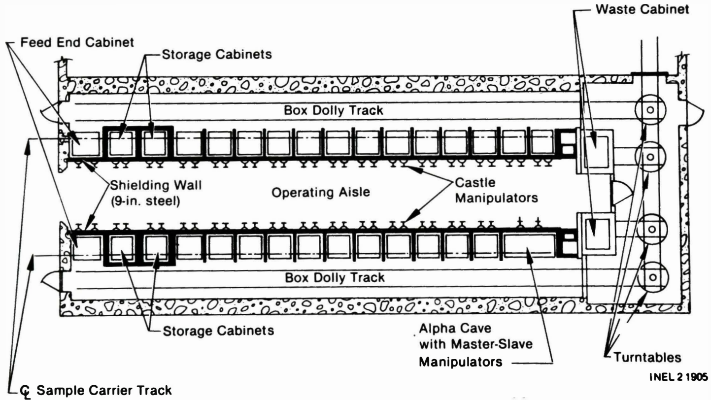
Figure 17. Plan view of the Remote Analytical Facility.
