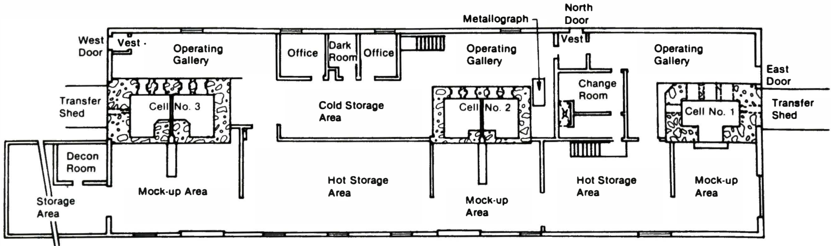
Figure 12. Plan view of TRA hot cells.
