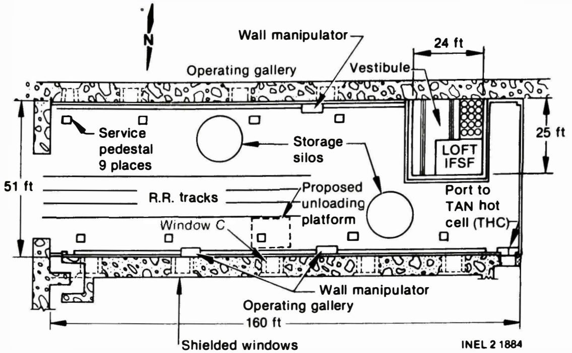
Figure 3. Plan view of TAN-607 Hot Shop.
