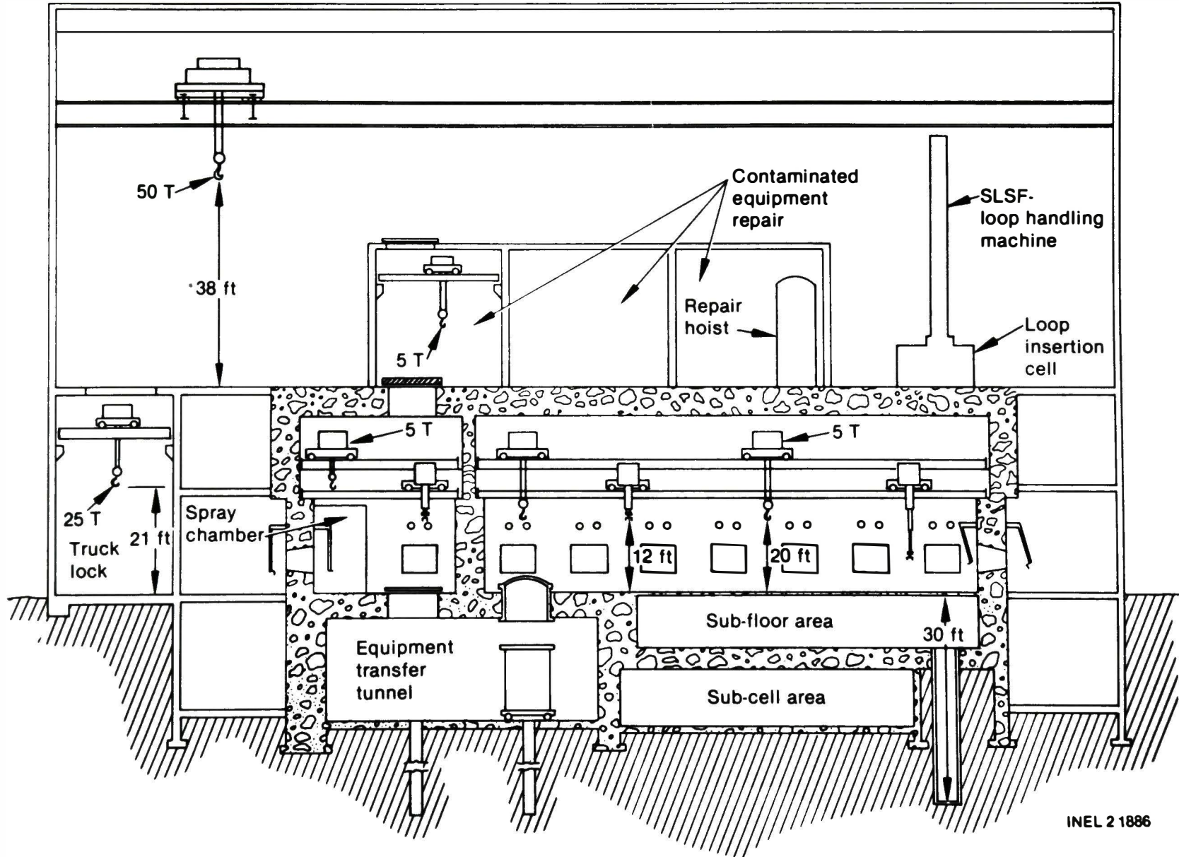
Figure 14. Elevation view of HFEF-N.
