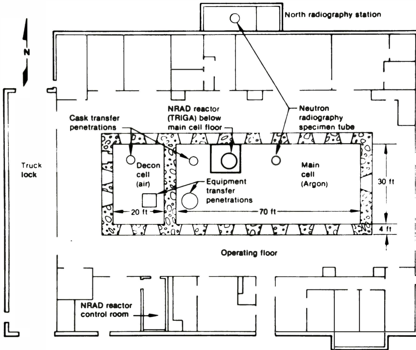
Figure 13. Plan view of HFEF-N.
