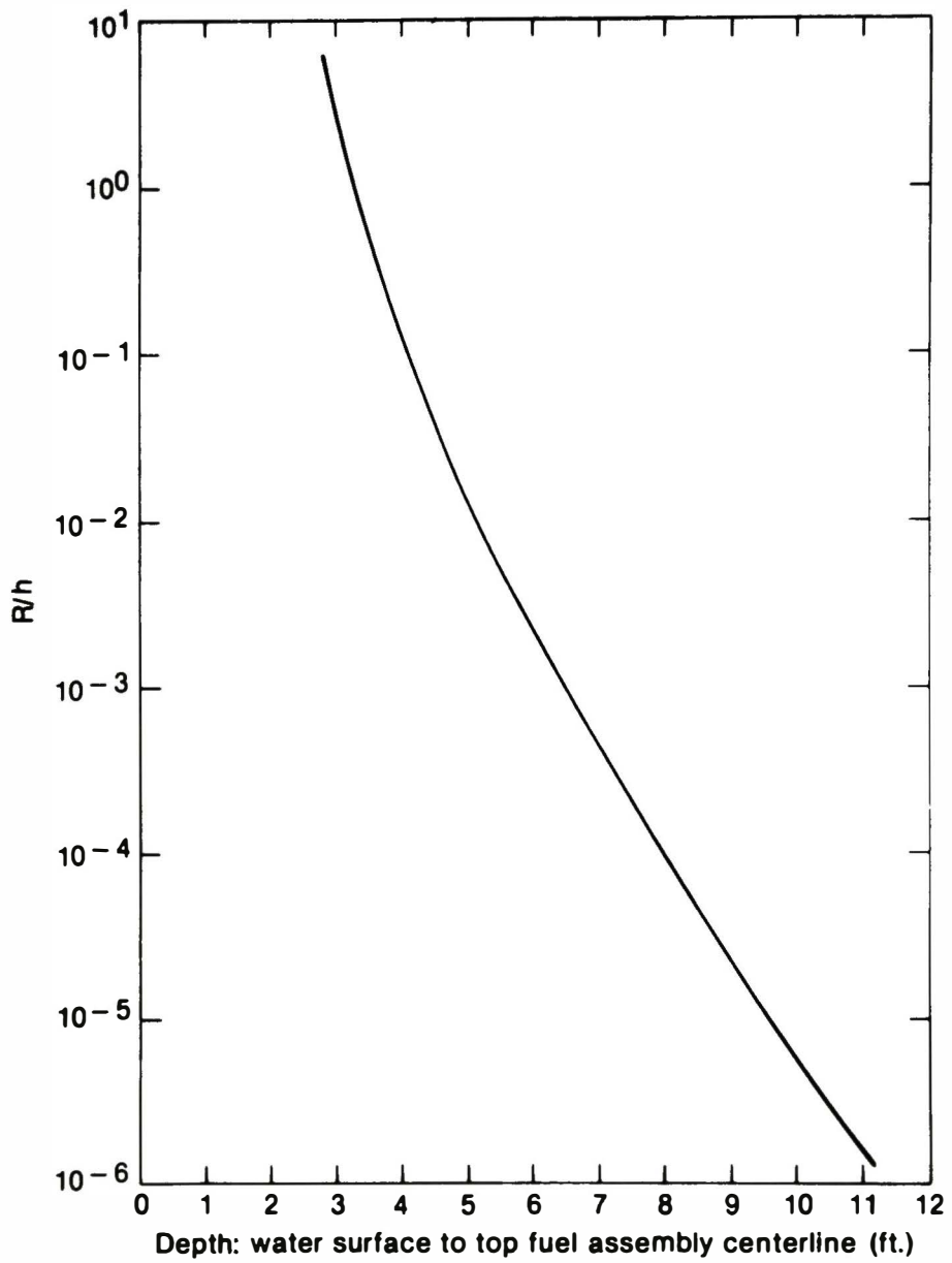
Figure B-1. Radiation field at a point 1 ft above the water surface.
