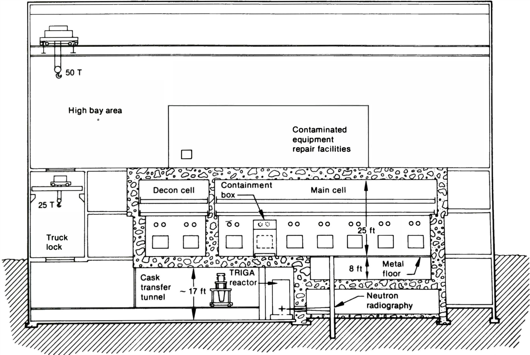
Figure 5. Elevation view of HFEF-N showing the cask transfer tunnel and neutron radiography facility.
