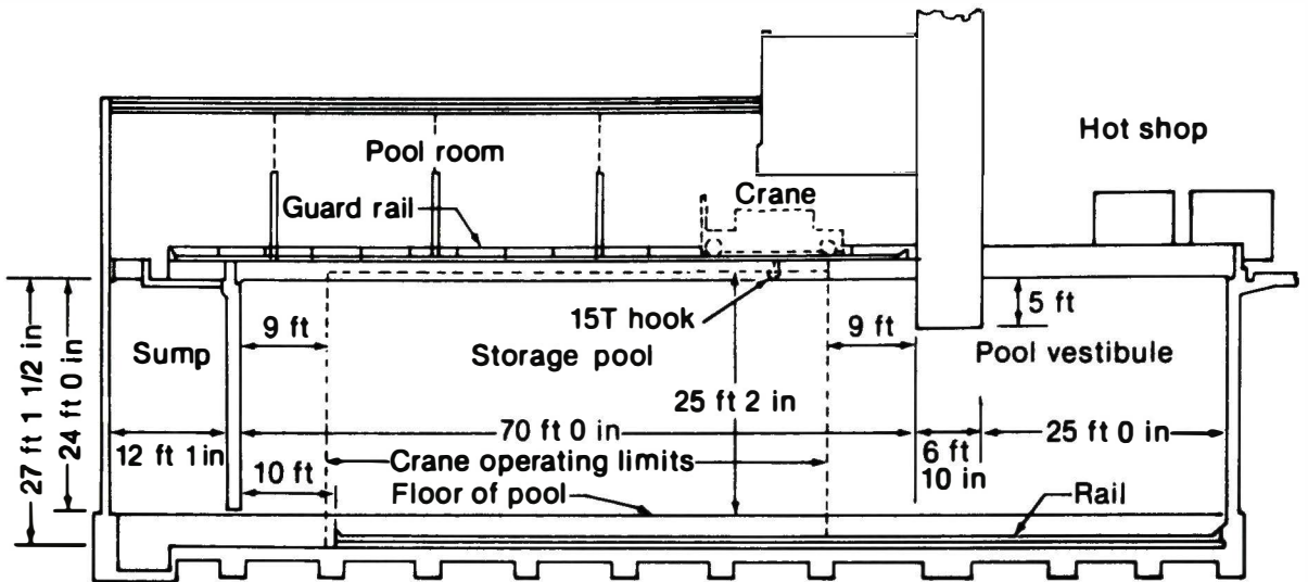
Figure 10. Elevation view of TAN-607 storage pool.
