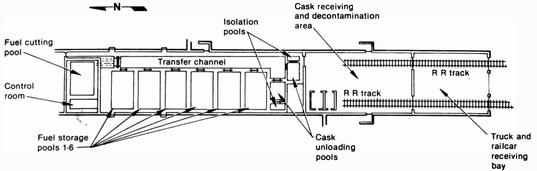
Figure 6. Plan view of FAST Fuel Storage Area (FSA).
