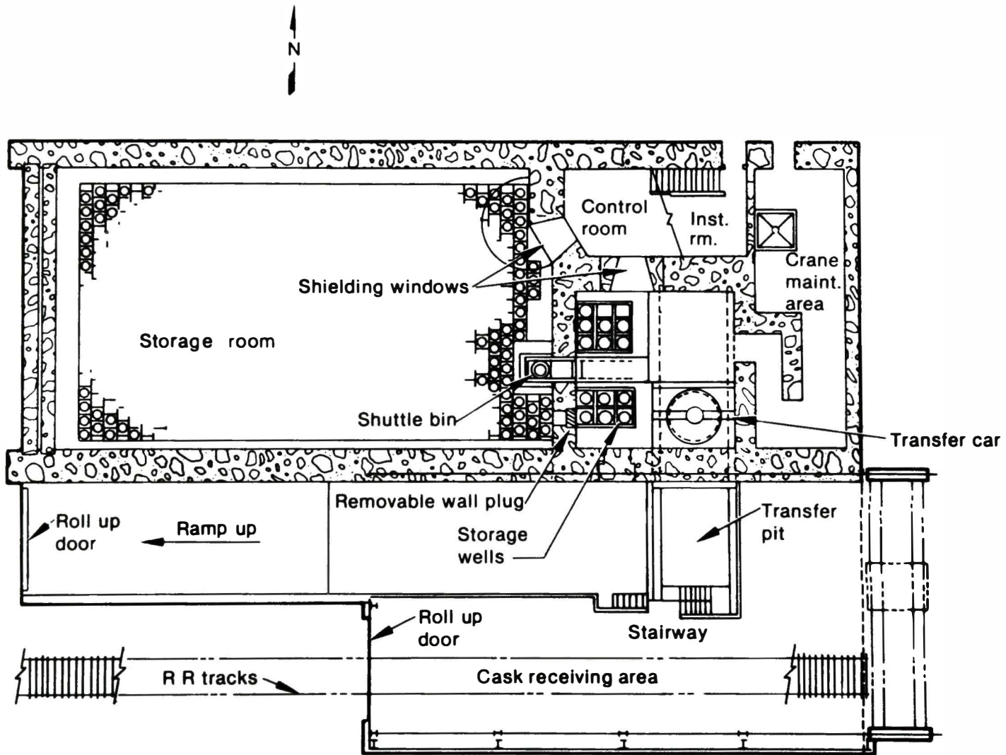
Figure 7. Plan view of the Irradiated Fuel Storage Facility (IFSF).
