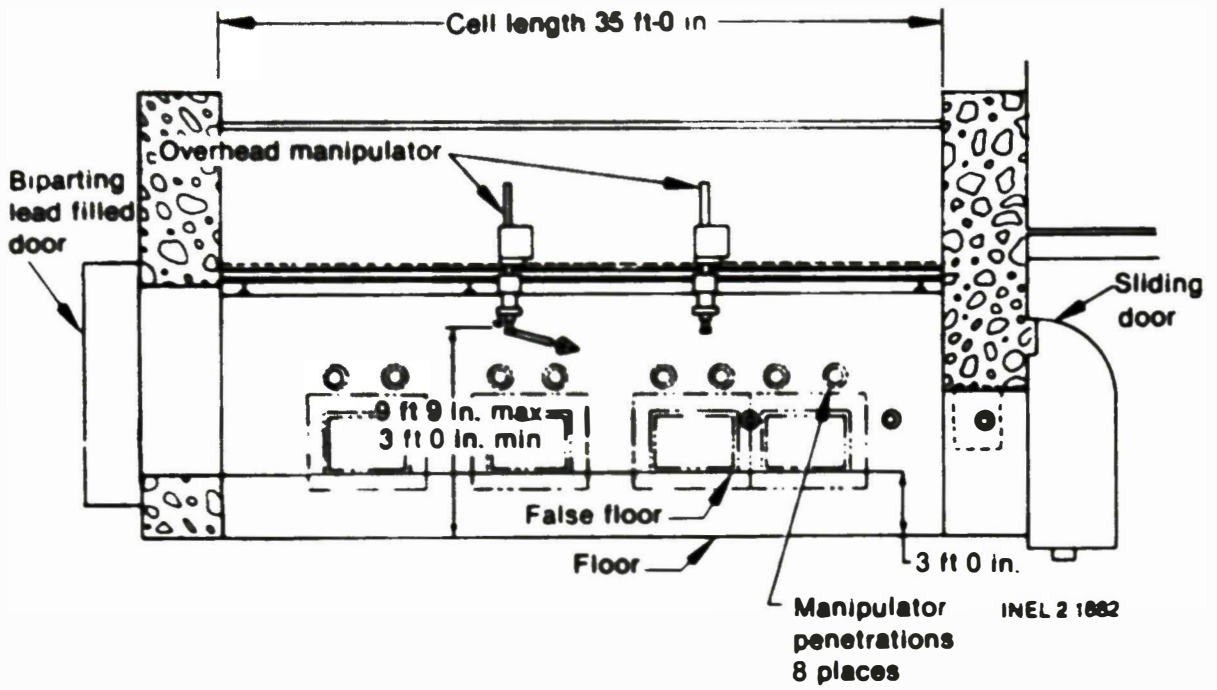
Figure 9. Elevation view of TAN-607 Hot Cell showing handling equipment.
