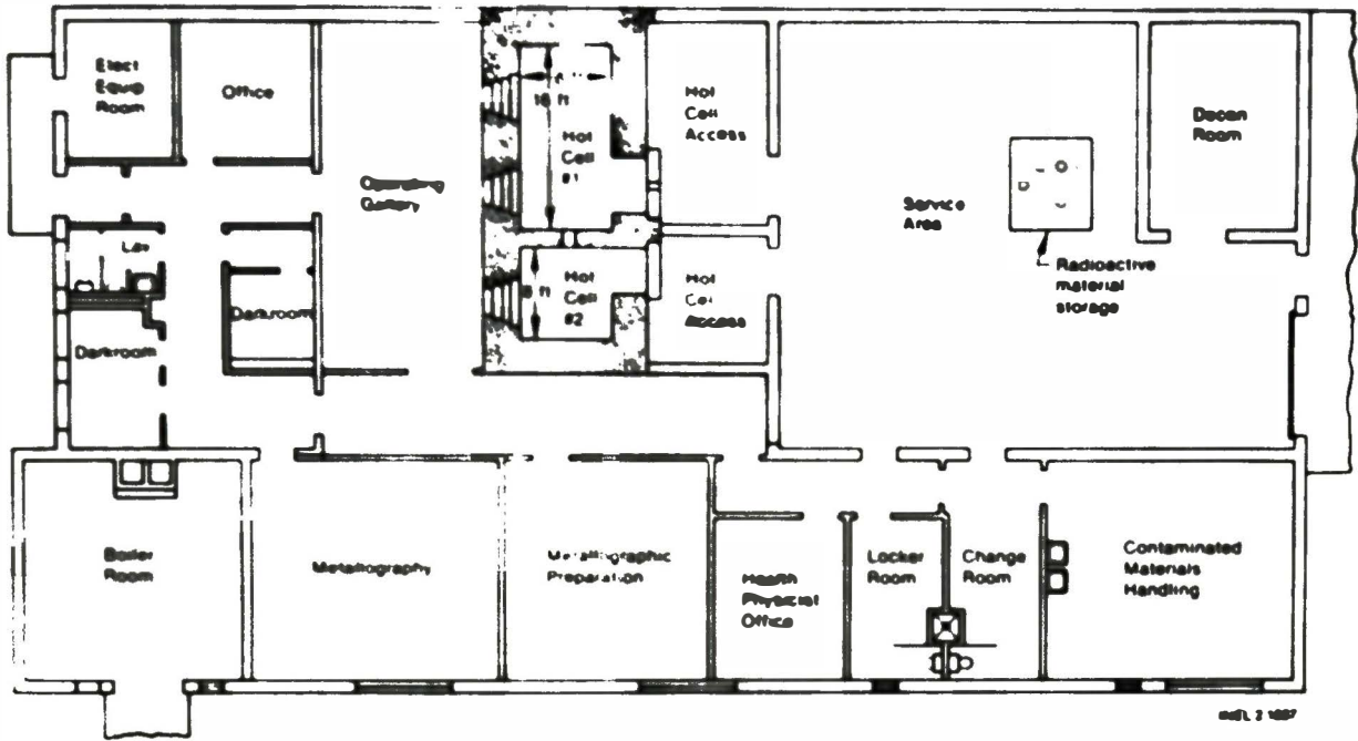
Figure 11. Plan view of ARA hot cells.
