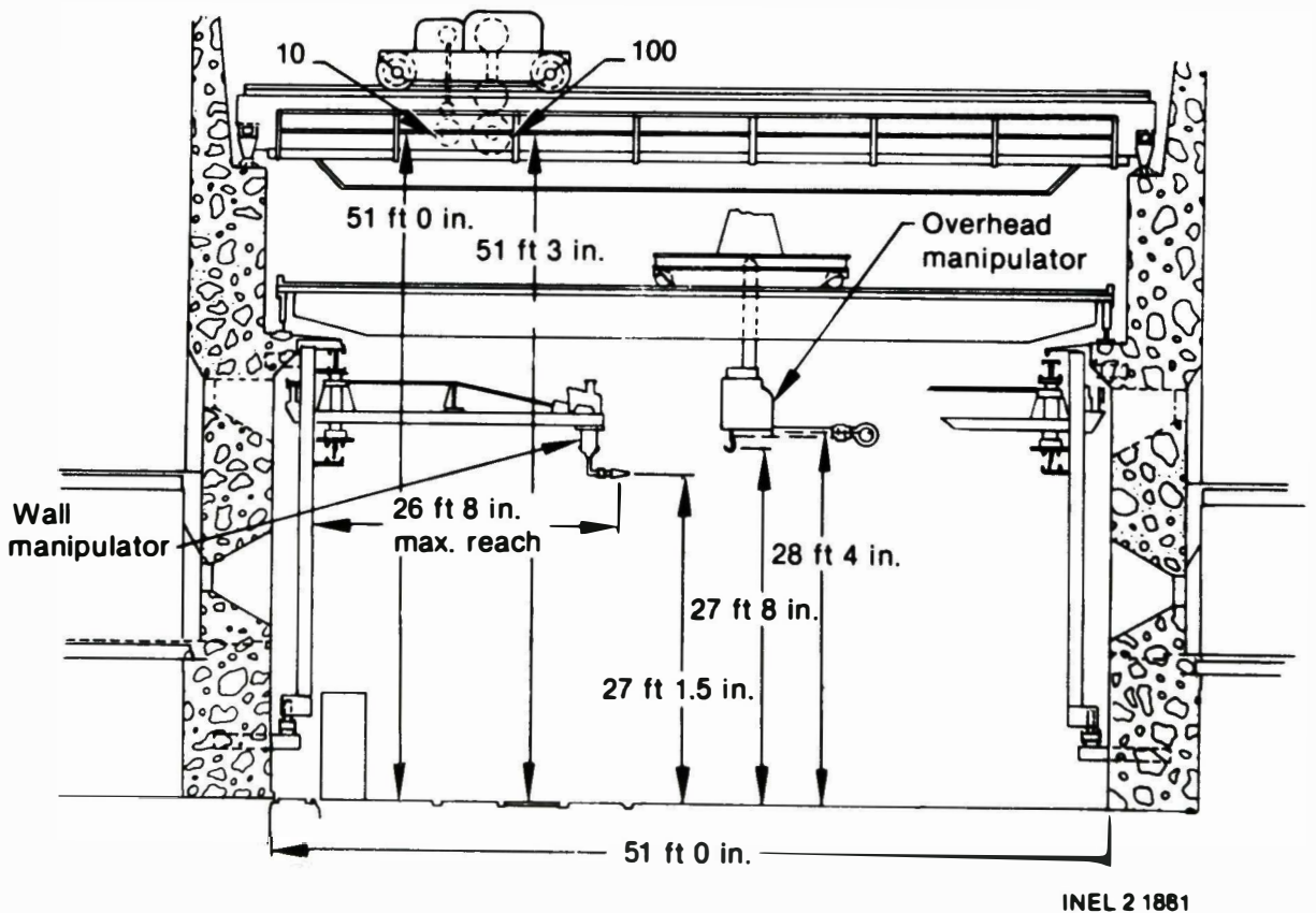
Figure 4. Elevation view of Hot Shop remote handling equipment.
