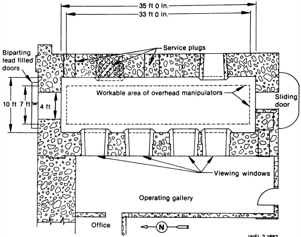
Figure 8. Plan view of TAN-607 Hot Cell (THC).
