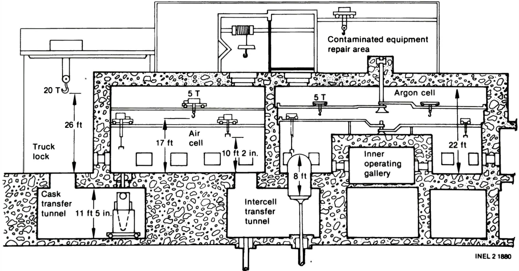
Figure 16. Elevation view of HFEF-S.
