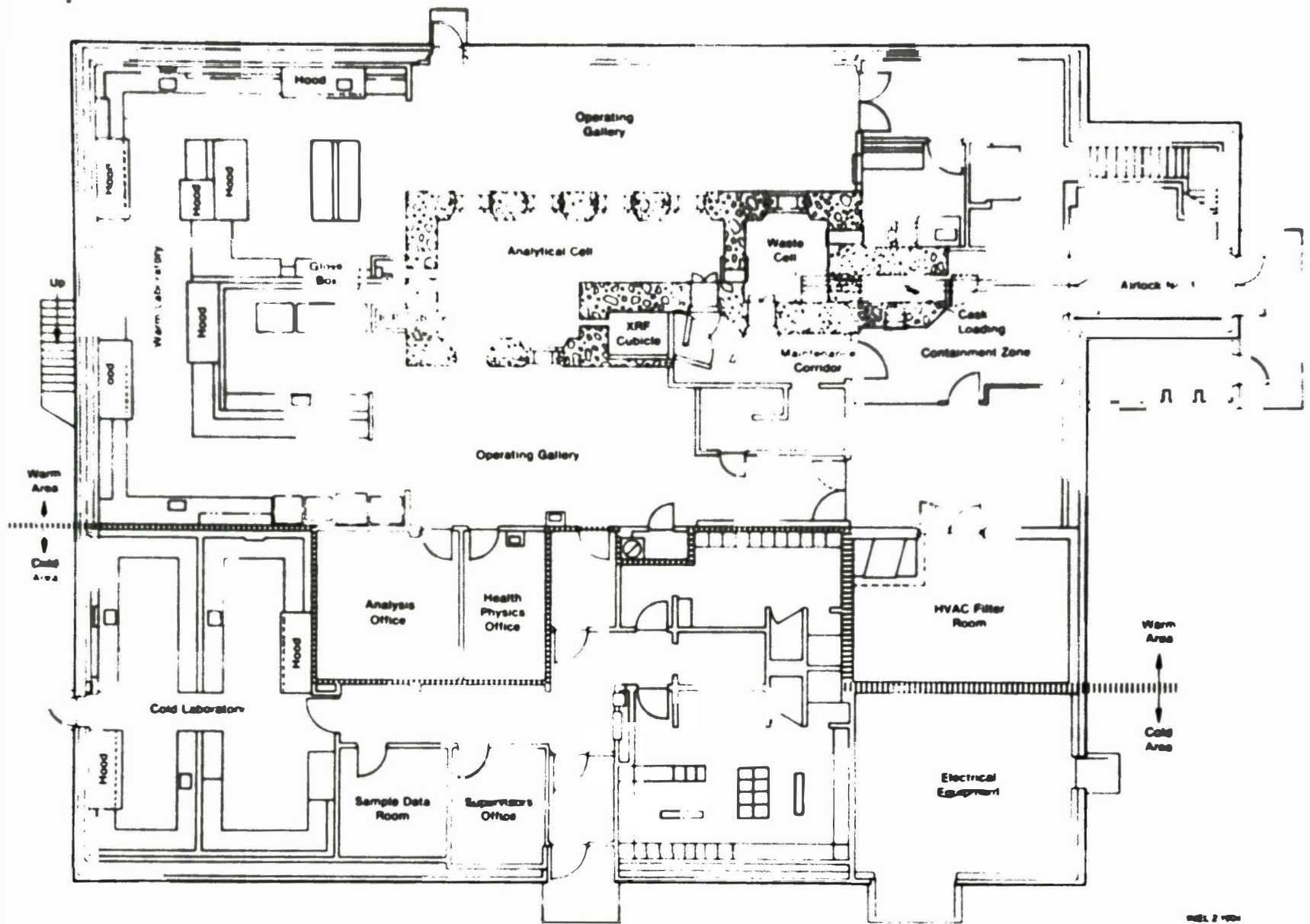
Figure 18. Plan view of the Remote Analytical Laboratory.
